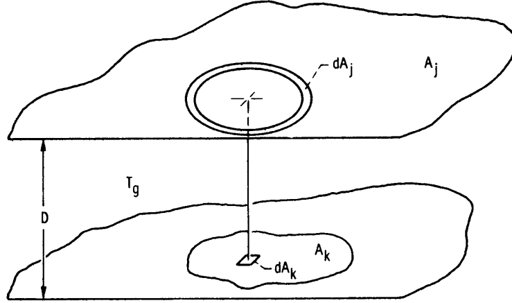
FIGURE B.5 Isothermal layer of medium between infinite parallel plates.
